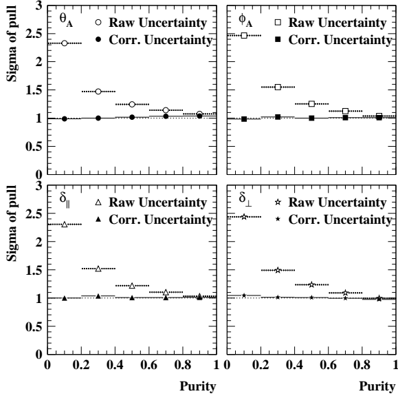
FIG. 17: Root mean square (RMS) of the pull distributions as a function of signal purity (defined in the 5.2 - 5.3 \text{ GeV}/c^2 m_{ES} range), for the fitted parameters \theta_A, \phi_A, \delta_{\parallel} , and \delta_{\perp} . Open symbols denote the RMS of the pulls computed with the uncertainties taken directly from Minuit . Closed symbols denote the uncertainties computed according to Eq. A1.
