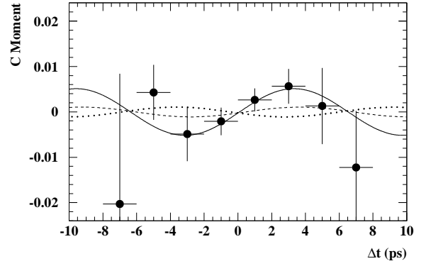
FIG. 12: The moment of \mathcal{C} as a function of \Delta t . The overlaid curve corresponds to the fit results (Table XI). The dashed curve corresponds to \cos 2\beta = +\sqrt{1 - \sin^2 2\beta_0} = +0.68 [4], the dotted one to the non-standard solution \cos 2\beta = -0.68 .
